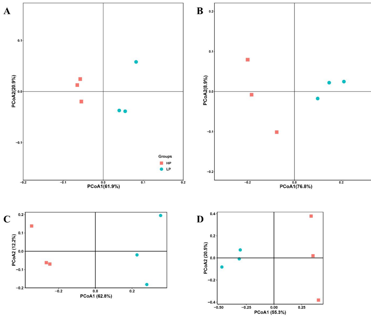
Fig. S2 Principal coordinates analysis (PCoA) of bacteria (A, C) and fungi (B, D) in rhizosphere soil (A, B) and root (C, D). (n = 3; “LP” represents zoysiagrass grown with ZS-1 strain invasion; “HP” represents zoysiagrass grown without ZS-1 strain invasion.)
