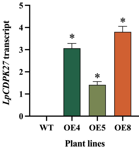
Figure S1. LpCDPK27 transcript levels in LpCDPK27 overexpressing Arabidopsis lines in comparison with the wild type (WT, Col-0) were analyzed. The asterisk indicates significant difference between transgenic lines and the wild-type at P < 0.05 .
