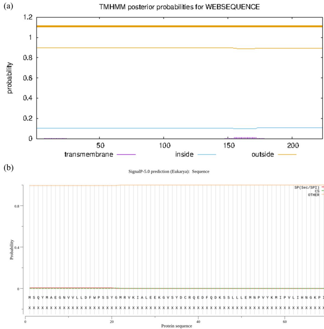
Supplemental Figure S2. The transmembrane domains and signal peptide analysis of MsGSTU17. (a) The transmembrane domains analysis of MsGSTU17. (b) The signal peptide analysis of MsGSTU17.
