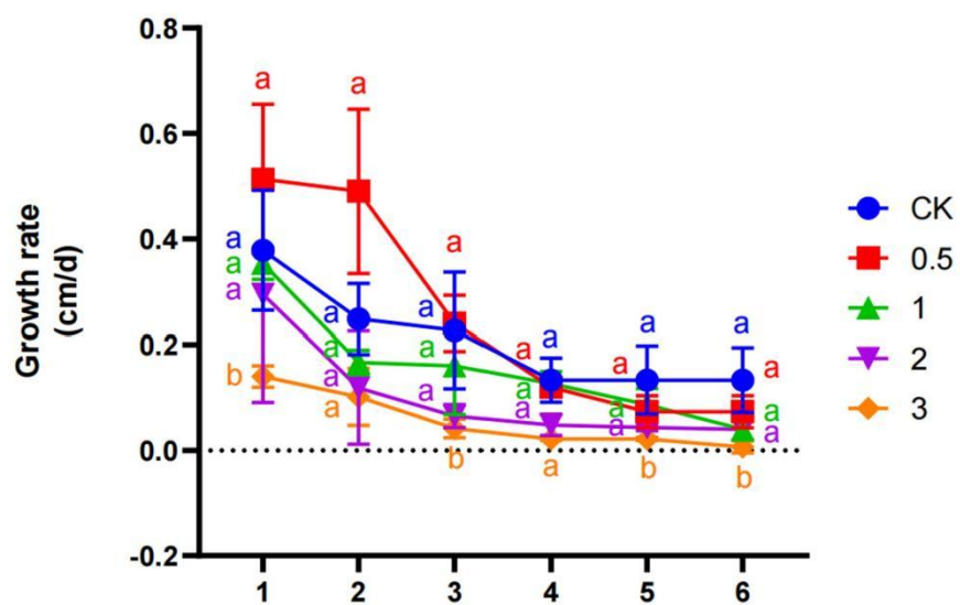
Figure S2 Effects of different concentrations of salt treatment on leaf growth rate of Festuca rubra
