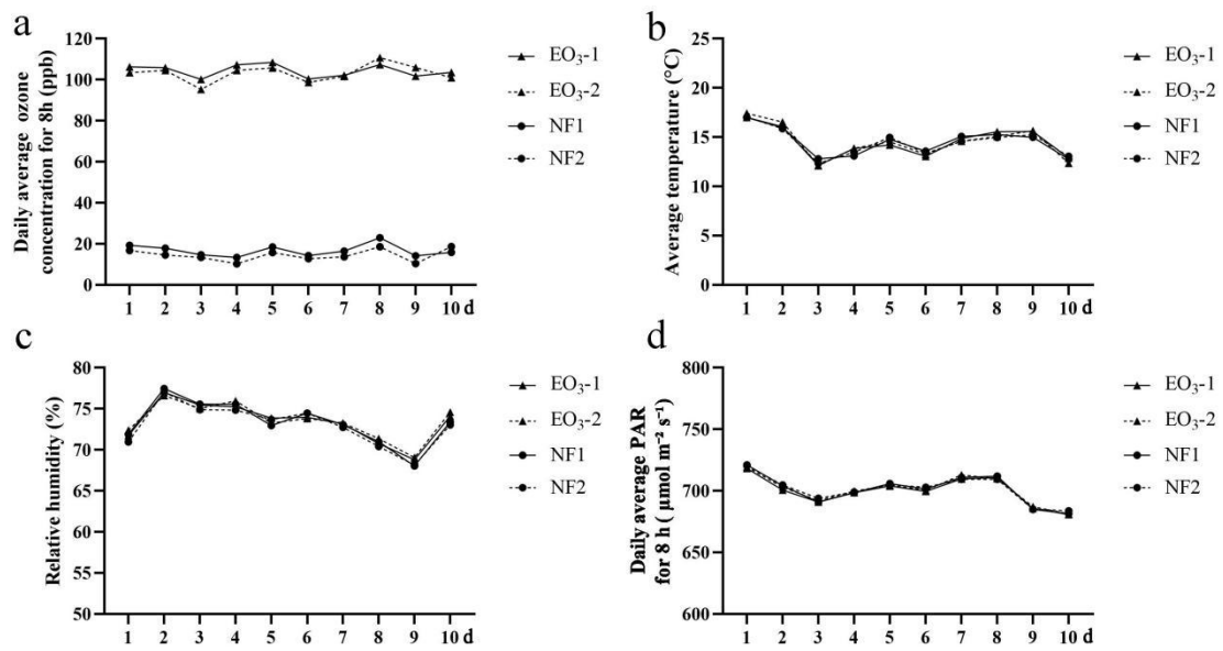
Figure S1 Daily average ozone concentration (a), temperature (b), relative humidity (c), and photosynthetically active radiation (PAR, d) for 8 hours (09:00 to 17:00) in OTCs under different treatments during the experiment. NF represents the non-filtered ambient air, and EO 3 represents ambient air adding 80 ppb ozone.
