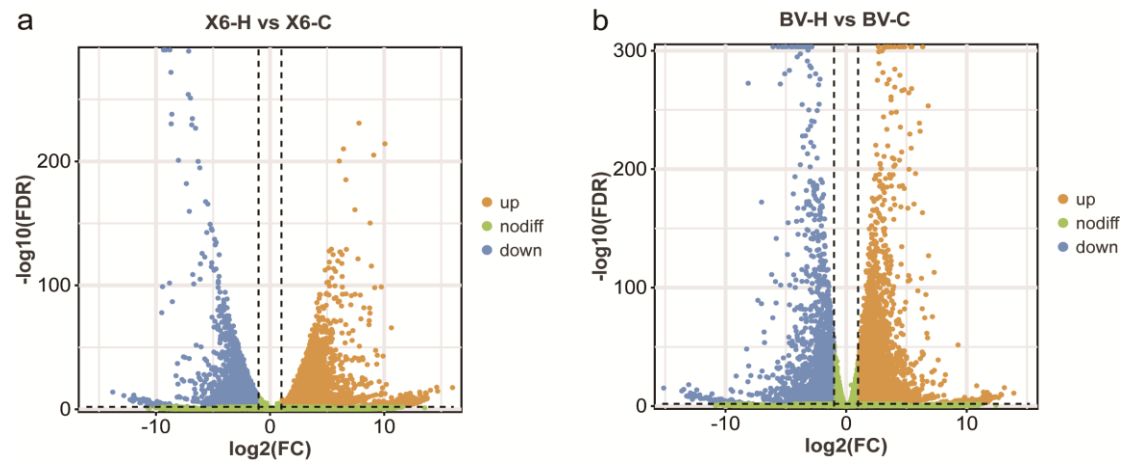
Supplementary Figure S3 Volcano plot for DEGs of two ryegrass varieties with contrasting heat tolerance. (a) X6-H vs X6-C; (b) BV-H vs BV-C.
