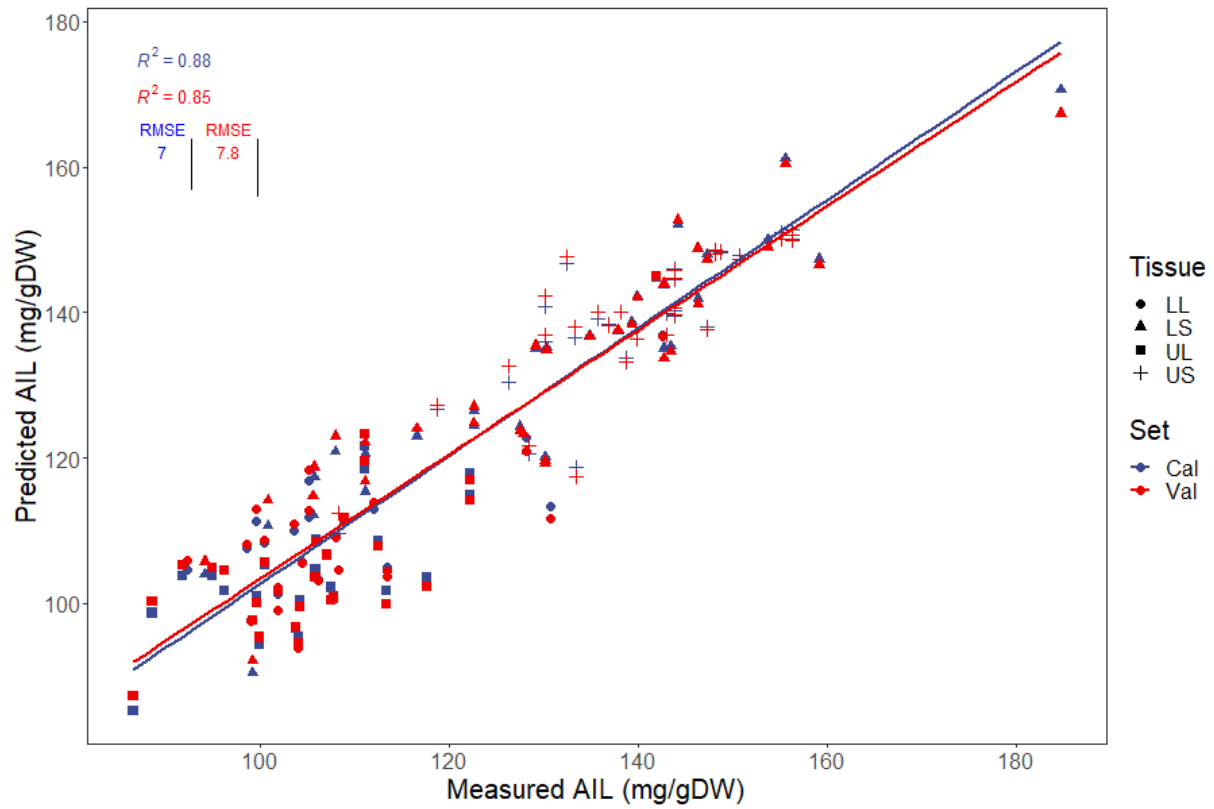
Supplementary Figure 10. PLSR models generated for predicting mg/g of biomass comprised of AIL present in four different tissues of multiple Cenchrus accessions; lower stem (LS), lower leaf (LL), upper stem (US) and upper leaf (UL). Plots show calibration predictions (cal) as well as cross-validated predictions (val) used to evaluate the accuracy of the model.
