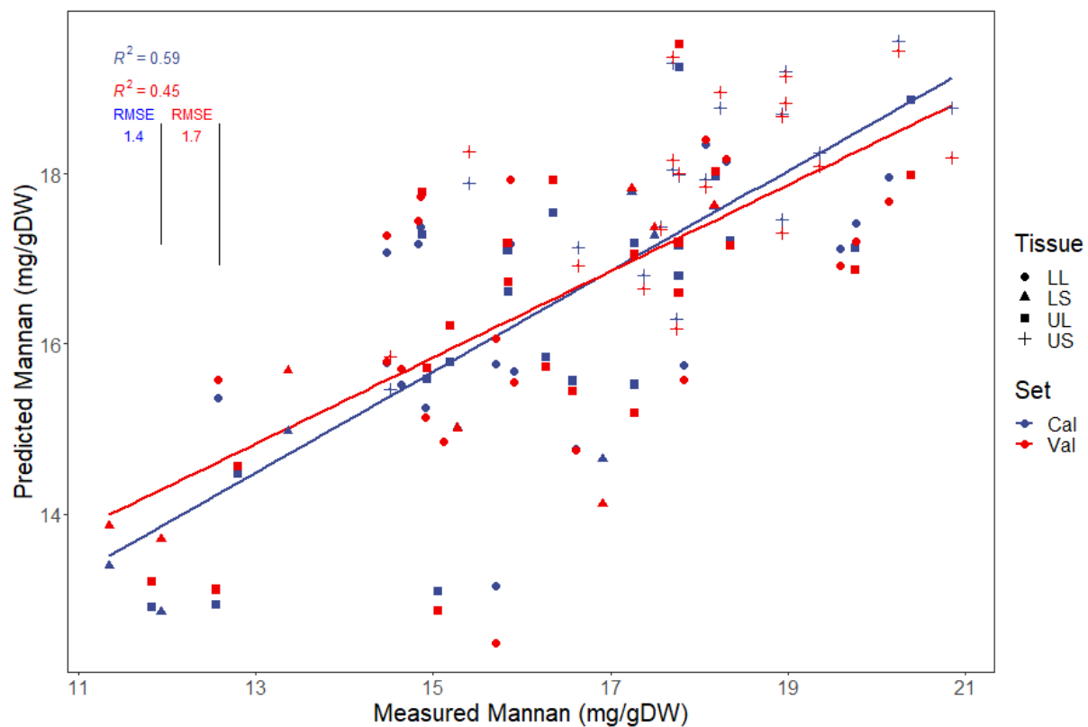
Supplementary Figure 9. PLSR models generated for predicting mg/g of biomass comprised of mannan present in four different tissues of multiple Cenchrus accessions; lower stem (LS), lower leaf (LL), upper stem (US) and upper leaf (UL). Plots show calibration predictions (cal) as well as cross-validated predictions (val) used to evaluate the accuracy of the model.
