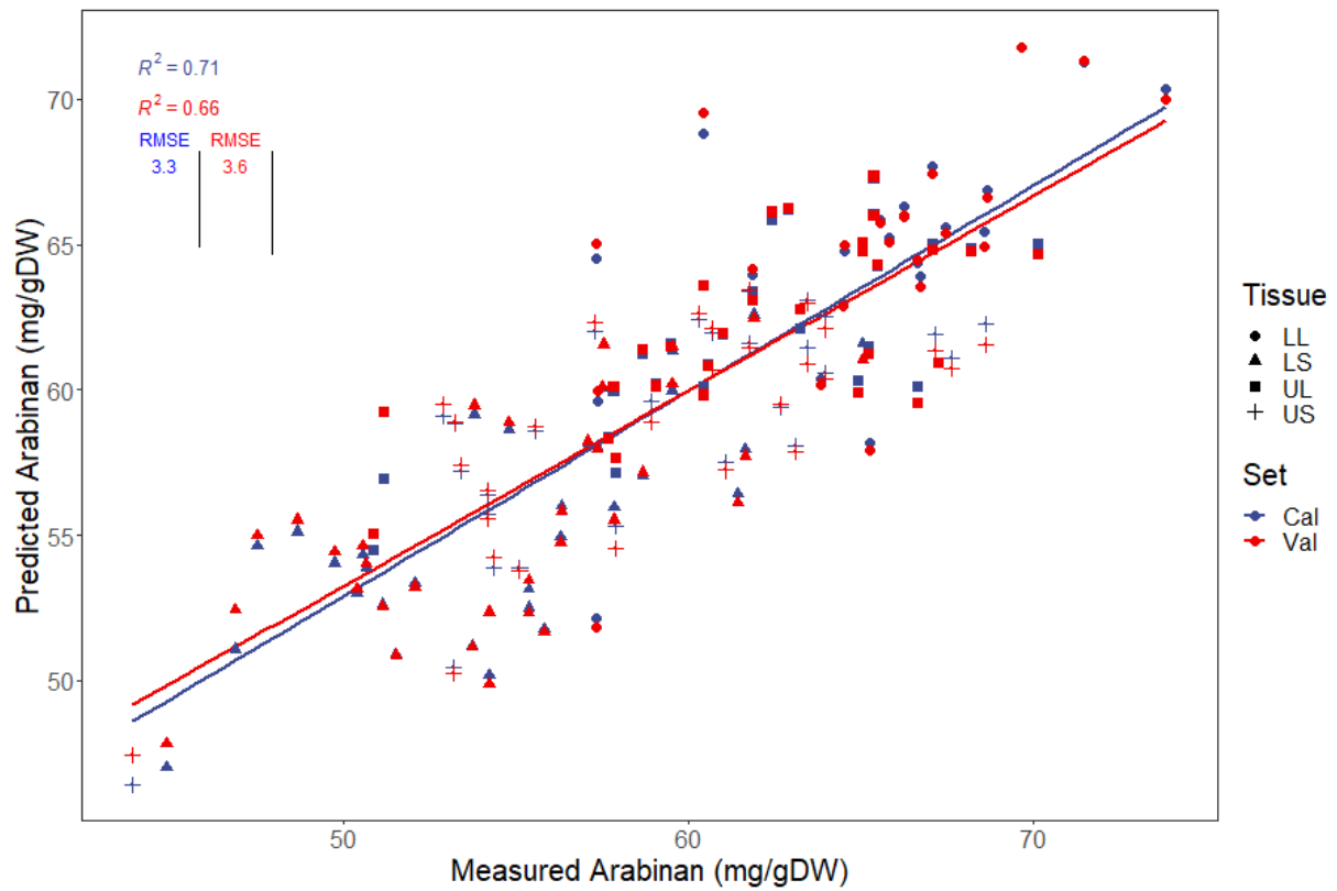
Supplementary Figure 8. PLSR models generated for predicting mg/g of biomass comprised of arabinan present in four different tissues of multiple Cenchrus accessions; lower stem (LS), lower leaf (LL), upper stem (US) and upper leaf (UL). Plots show calibration predictions (cal) as well as cross-validated predictions (val) used to evaluate the accuracy of the model.
