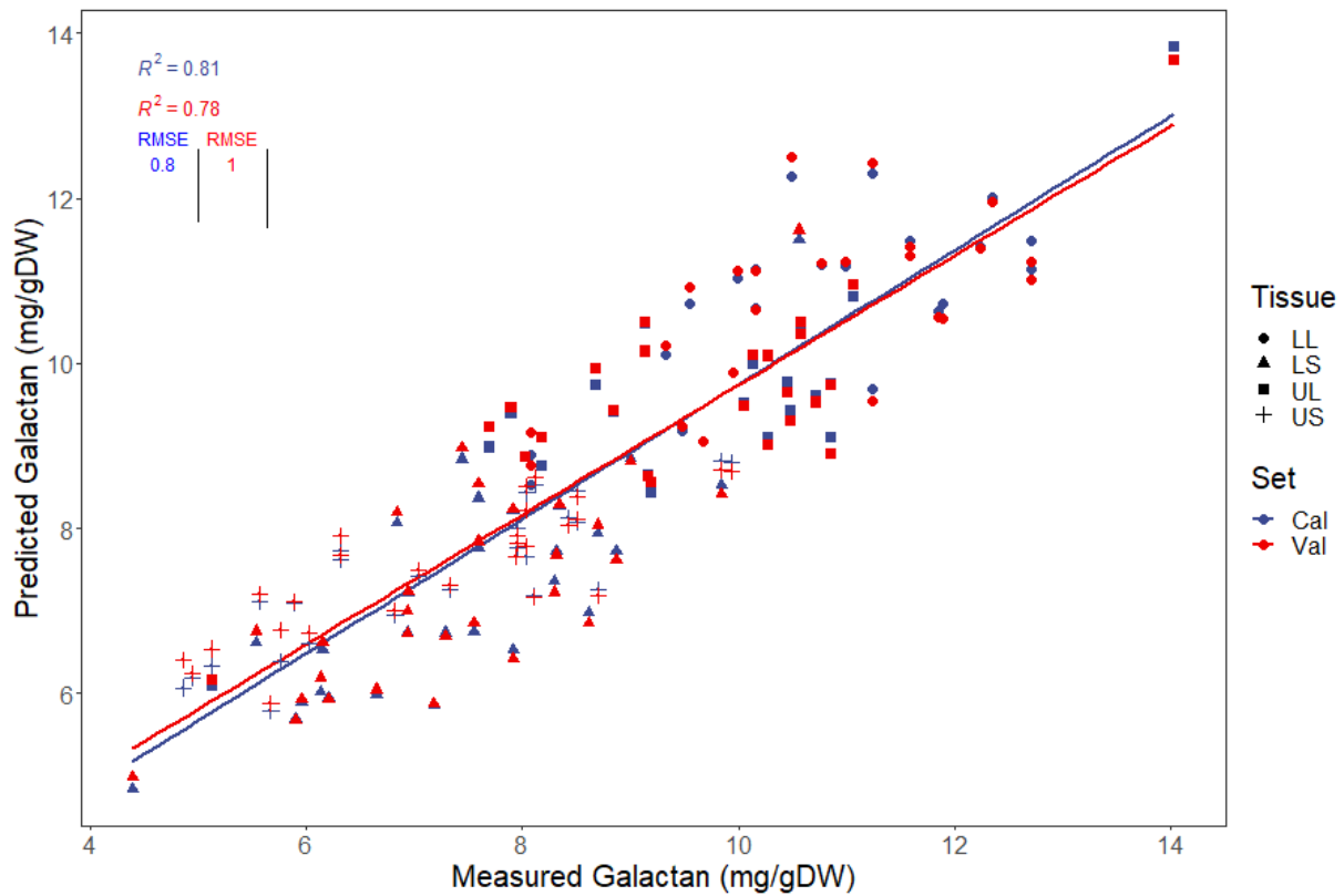
Supplementary Figure 7. PLSR models generated for predicting mg/g of biomass comprised of galactan present in four different tissues of multiple Cenchrus accessions; lower stem (LS), lower leaf (LL), upper stem (US) and upper leaf (UL). Plots show calibration predictions (cal) as well as cross-validated predictions (val) used to evaluate the accuracy of the model.
