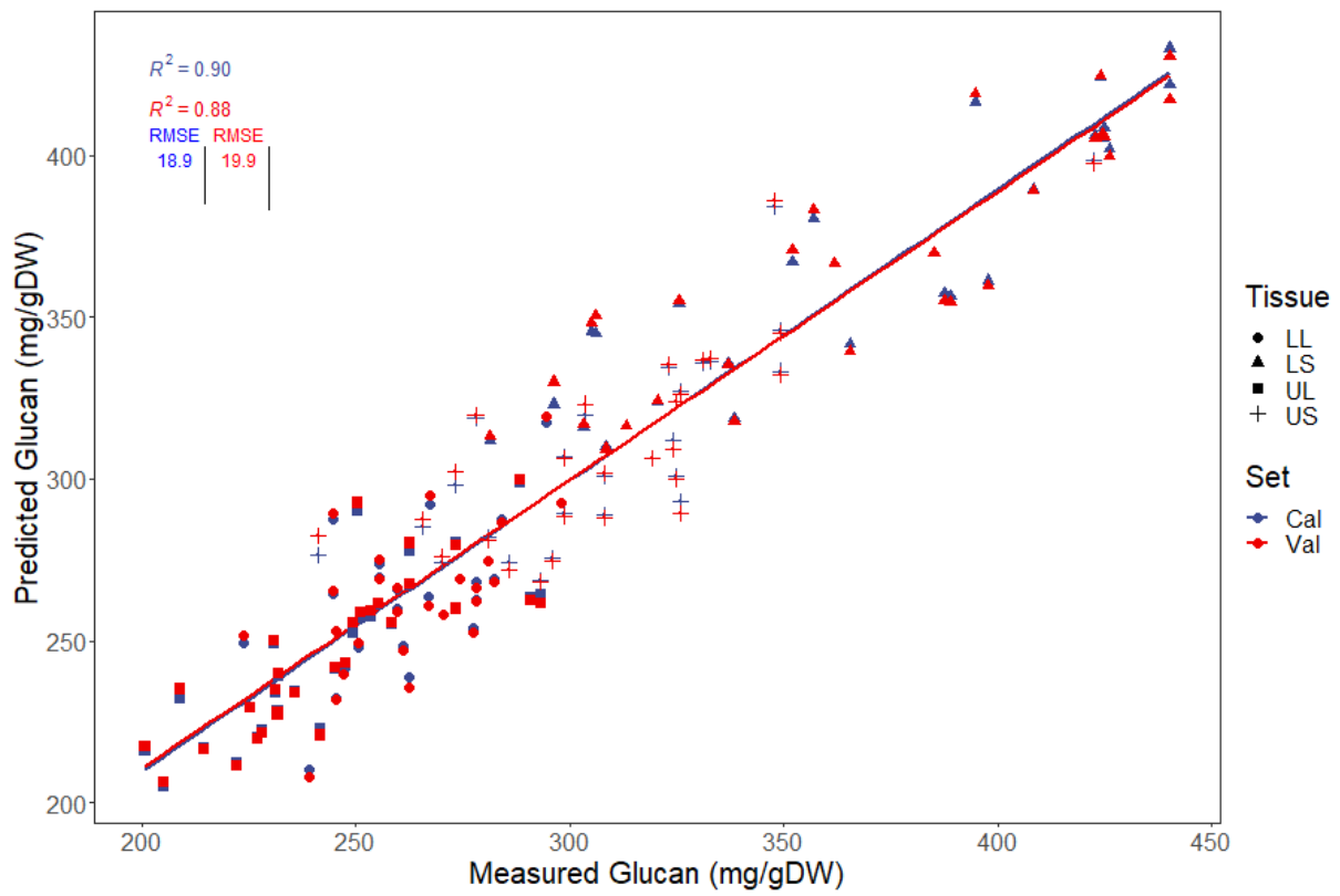
Supplementary Figure 5. PLSR models generated for predicting mg/g of biomass comprised of glucan present in four different tissues of multiple Cenchrus accessions; lower stem (LS), lower leaf (LL), upper stem (US) and upper leaf (UL). Plots show calibration predictions (cal) as well as cross-validated predictions (val) used to evaluate the accuracy of the model.
