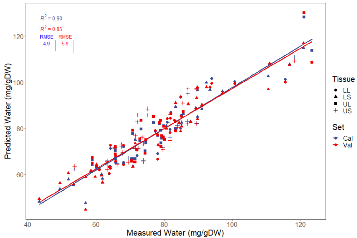
Supplementary Figure 4. PLSR models generated for predicting mg/g of biomass comprised of water present in four different tissues of multiple Cenchrus accessions; lower stem (LS), lower leaf (LL), upper stem (US) and upper leaf (UL). Plots show calibration predictions (cal) as well as cross-validated predictions (val) used to evaluate the accuracy of the model.
