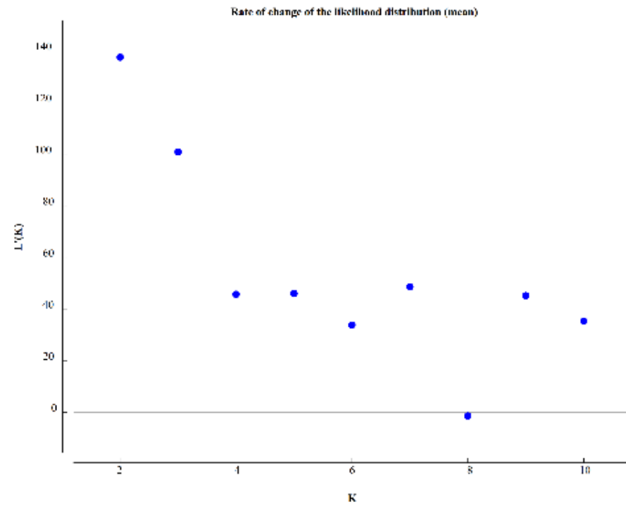
Supplemental Fig S3, STRUCTURE analysis, DeltaK and rate of change of the likelihood distribution.
