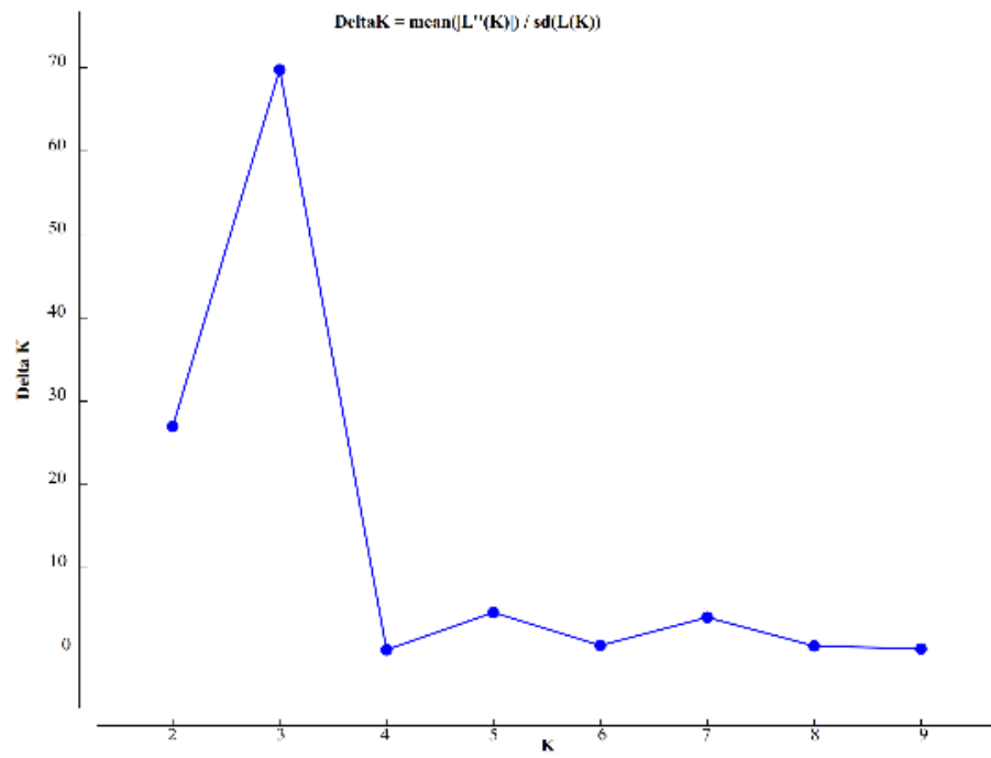
Supplemental Fig S3, STRUCTURE analysis, DeltaK and rate of change of the likelihood distribution.
