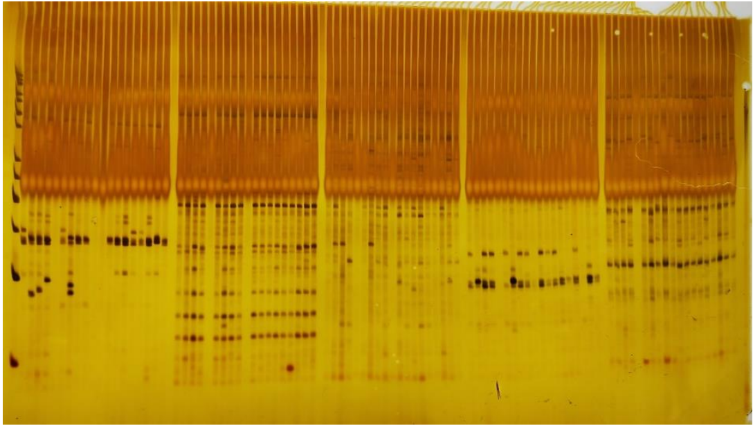
Supplemental Fig S2. Polymorphism primer gel of SSR1-SSR5
