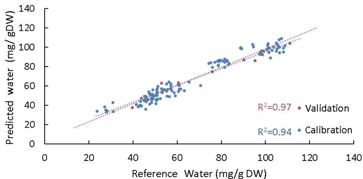
Supplementary Figure 3. Predicted water content of the cell wall value determined by PLSR model generated from FTIR Spectra vs reference values water extracted by freeze drying ground leaf clippings obtained from Cynodon grasses including the R^2 and RMSE for a calibration and validation set of samples. The calibration set (blue) was used to generate the model, while another independent validation set (red) was used to test its ability to predict unknown datasets. The R^2 and RMSE obtained for the validation set measured the model's effectiveness for predicting unknown samples based on their FTIR spectra.
