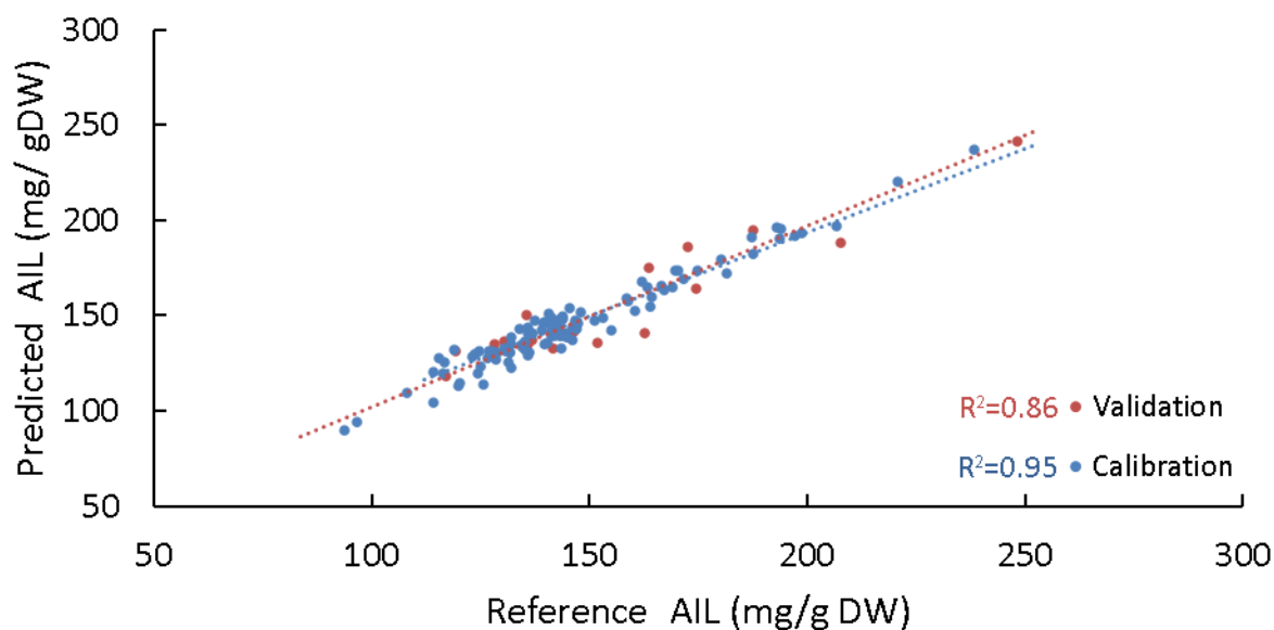
Supplementary Figure 10 Predicted Cell wall values determined by PLSR model generated from FTIR Spectra vs reference AIL values extracted from cell wall isolated from dried ground leaf clippings obtained from Cynodon grasses including the R 2 and RMSE for a calibration and validation set of samples. The calibration set (blue) was used to generate the model, while another independent validation set (red) was used to test its ability to predict unknown datasets. The R 2 and RMSE obtained for the validation set measured the model's effectiveness for predicting unknown samples based on their FTIR spectra.
