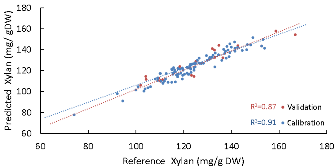
Supplementary Figure 6 Predicted Cell wall values determined by PLSR model generated from FTIR Spectra vs reference xylan values extracted from cell wall isolated from dried ground leaf clippings obtained from Cynodon grasses including the R 2 and RMSE for a calibration and validation set of samples. The calibration set (blue) was used to generate the model, while another independent validation set (red) was used to test its ability to predict unknown datasets. The R 2 and RMSE obtained for the validation set measured the model's effectiveness for predicting unknown samples based on their FTIR spectra.
