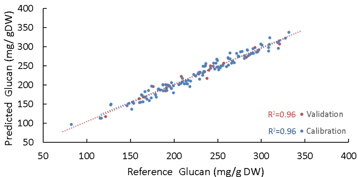
Supplementary Figure 5 Predicted Cell wall values determined by PLSR model generated from FTIR Spectra vs reference glucan values extracted from cell wall isolated from dried ground leaf clippings obtained from Cynodon grasses including the R 2 and RMSE for a calibration and validation set of samples. The calibration set (blue) was used to generate the model, while another independent validation set (red) was used to test its ability to predict unknown datasets. The R 2 and RMSE obtained for the validation set measured the model's effectiveness for predicting unknown samples based on their FTIR spectra.
