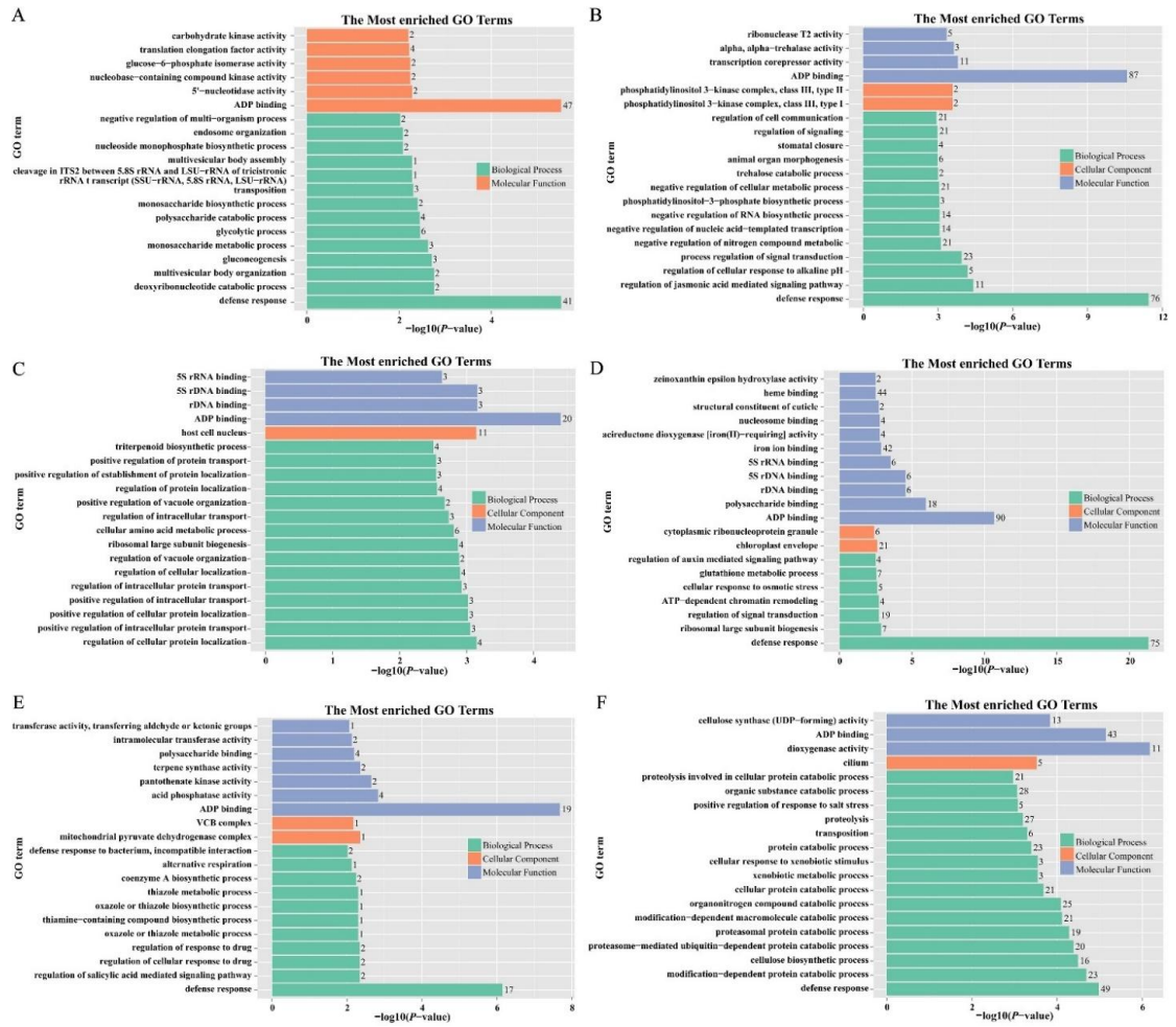
Fig. S5 GO enrichment of sex-specific genes. (A) Genes present only in female plants. (B) Genes absent in female plants. (C) Genes present only in male plants. (D) Genes absent in male plants. (E) Genes present only in monoecious plants. (F) Genes absent in monoecious plants.
