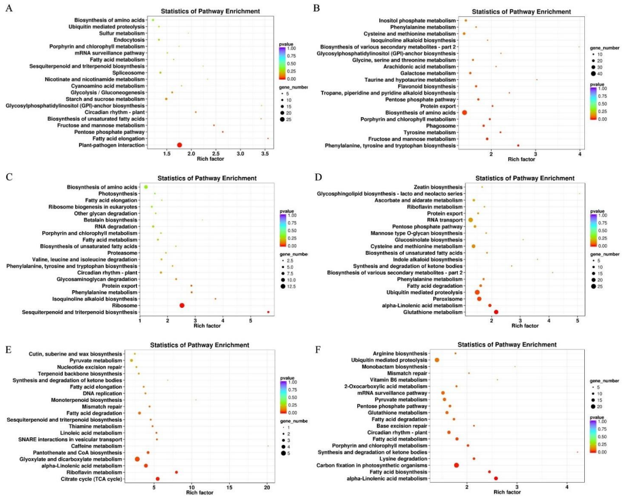
Fig. S6 KEGG enrichment of sex-specific genes. (A) Genes present only in female plants. (B) Genes absent in female plants. (C) Genes present only in male plants. (D) Genes absent in male plants. (E) Genes present only in monoecious plants. (F) Genes absent in monoecious plants.
