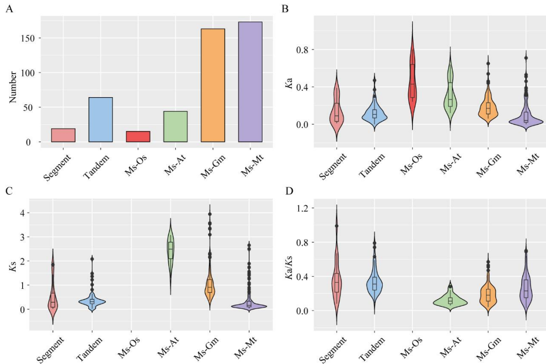
Figure S2. Ka and Ks analysis of plant CYP450 duplicated genes. The number (A), Ka (B), Ks (C), and Ka/Ks (D) of CYP450 duplicated genes. Segment, segmental duplicated gene pairs; tandem, tandem duplicated gene pairs; Ms-Os, CYP450 duplicated gene pairs between alfalfa and rice; Ms-At, CYP450 duplicated gene pairs between alfalfa and Arabidopsis; Ms-Gm, CYP450 duplicated gene pairs between alfalfa and soybean; Ms-Mt, duplicated gene pairs between alfalfa and thistle alfalfa.
