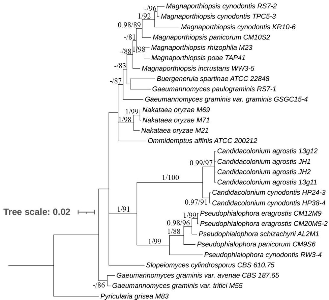
Fig. S5. Majority rule Bayesian phylogenetic tree derived from TEF1 DNA sequence data sets. Nodes having Bayesian inference posterior probabilities \geq 0.95 and maximum likelihood bootstrap values \geq 75\% are shown. The tree is rooted with Pyricularia grisea M83.
