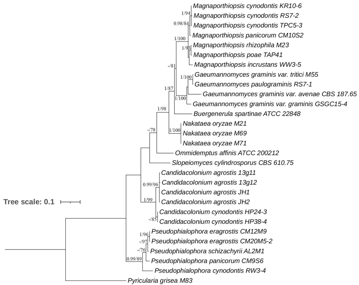
Fig. S4. Majority rule Bayesian phylogenetic tree derived from RPBI DNA sequence data sets. Nodes having Bayesian inference posterior probabilities \geq 0.95 and maximum likelihood bootstrap values \geq 75\% are shown. The tree is rooted with Pyricularia grisea M83.
