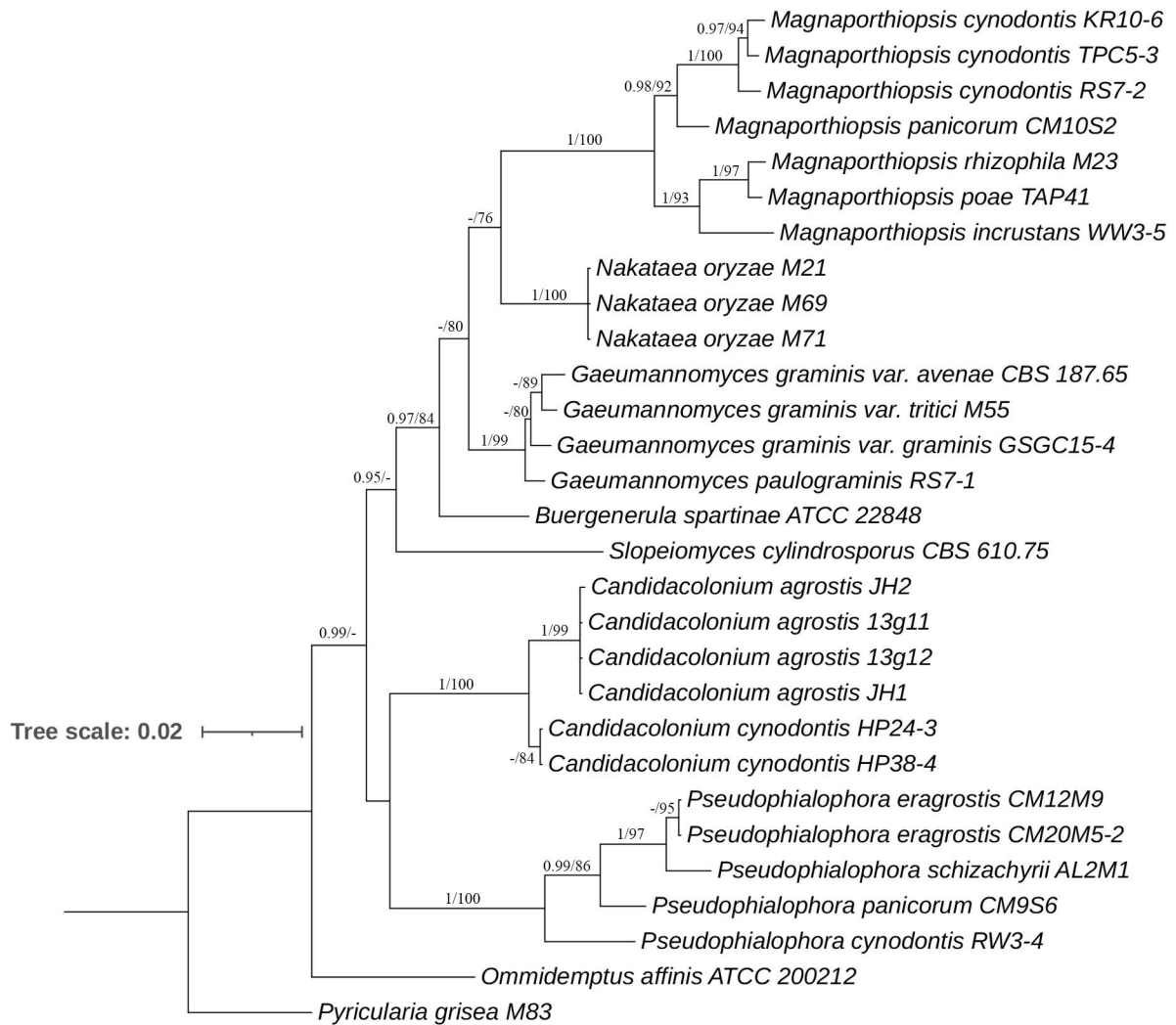
Fig. S2. Majority rule Bayesian phylogenetic tree derived from rDNA (the combined ITS, LSU and SSU) DNA sequence data sets. Nodes having Bayesian inference posterior probabilities \geq 0.95 and maximum likelihood bootstrap values \geq 75\% are shown. The tree is rooted with Pyricularia grisea M83.
