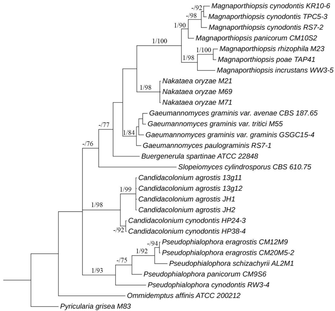
Fig. S1. Majority rule Bayesian phylogenetic tree derived from ITS DNA sequence data sets. Nodes having Bayesian inference posterior probabilities \geq 0.95 and maximum likelihood bootstrap values \geq 75\% are shown. The tree is rooted with Pyricularia grisea M83.
