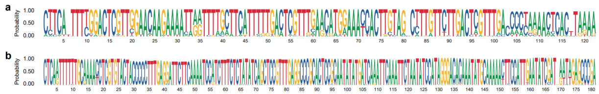
Supplementary Fig. 6 Logo plots of the two major tandem repeat units identified in the genome of C. monnieri . (a) The 118-bp monomer ( Cmon118 ) is the potentially primary centromeric satellite repeat. (b) The 180-bp monomer ( Cmon180 ) is likely a subtelomeric satellite repeat.
