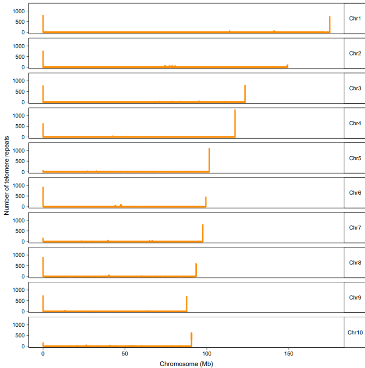
Supplementary Fig. 5 Distribution of telomere repeats along the genome of C. monnieri . Telomeres were identified using seven-base telomere repeats (5'-TTTAGGG-3') as sequence queries. Window size is 10 kb. Chromosomes 1-10 of the C. monnieri genome are shown.
