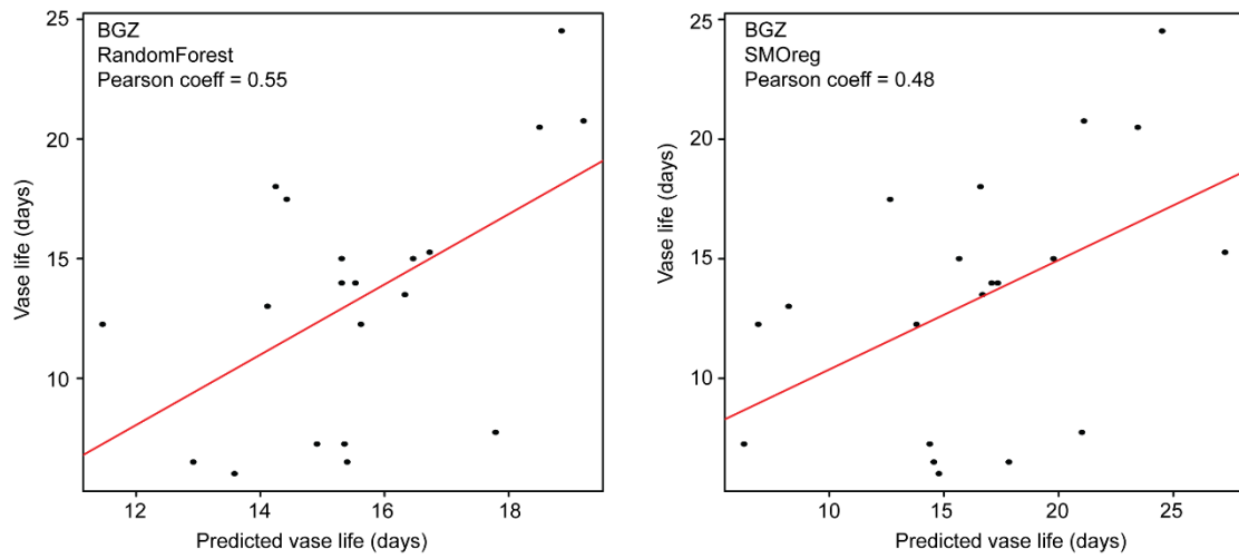
Fig. S3, Leaf vase life prediction using simple machine learning models. Scatterplots of predicted values versus manual measurements values of RandomForest (Left) and SMOreg algorithms.
