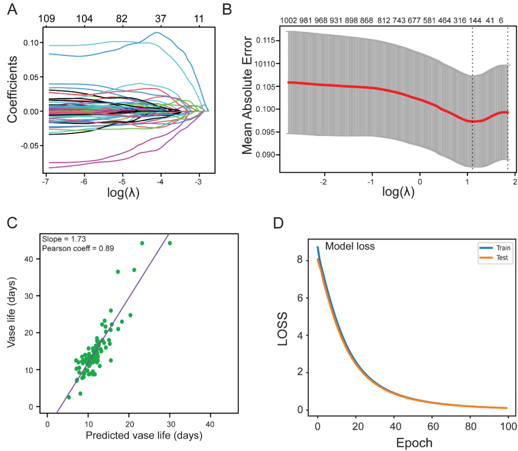
Fig. S2, Feature selection using LASSO algorithm. (A) The LASSO coefficient profiles. (B) Ten-time cross-validation for tuning parameter selection in the LASSO model. (C) Scatterplots between the predicted values and measured values. (D) The loss curve of the training and testing data for the deep learning model.
