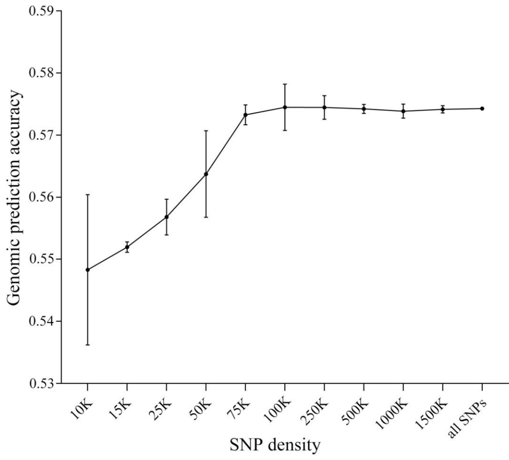
Figure S1. Genomic prediction accuracy at different SNP densities.
