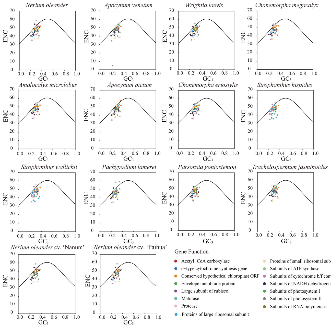
Figure S2. ENC versus GC 3 s relationship for protein-coding genes in 14 chloroplast genomes. Each point represents an individual gene, with the point size proportional to its ENC value. The solid black line represents the theoretical neutral expectation curve, where codon preference is determined exclusively by GC 3 s composition.
