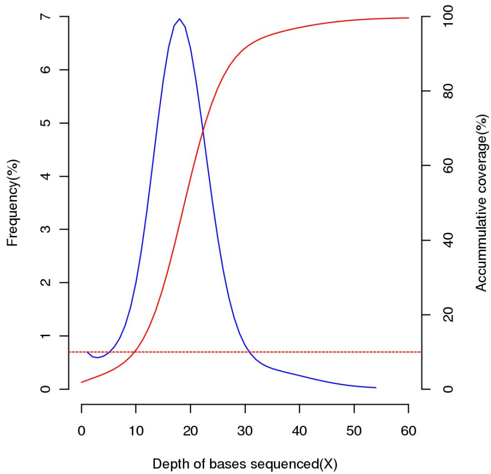
Supplemental Figure S1: Sequencing depth and cumulative coverage distribution of Illumina short reads mapped to the assembled genome.
