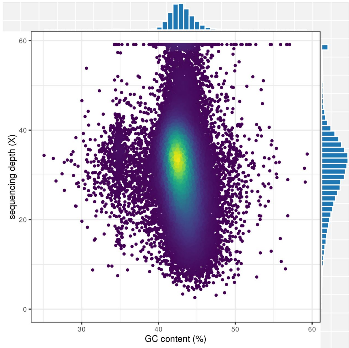
Supplemental Figure S2: GC content versus sequencing depth distribution across the assembled genome.
