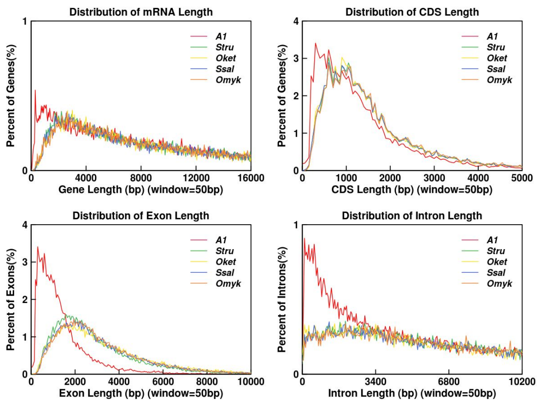
Supplemental Figure S3: Comparative distribution of gene structural features between Brachymystax lenok tsinlingensis and closely related species.
