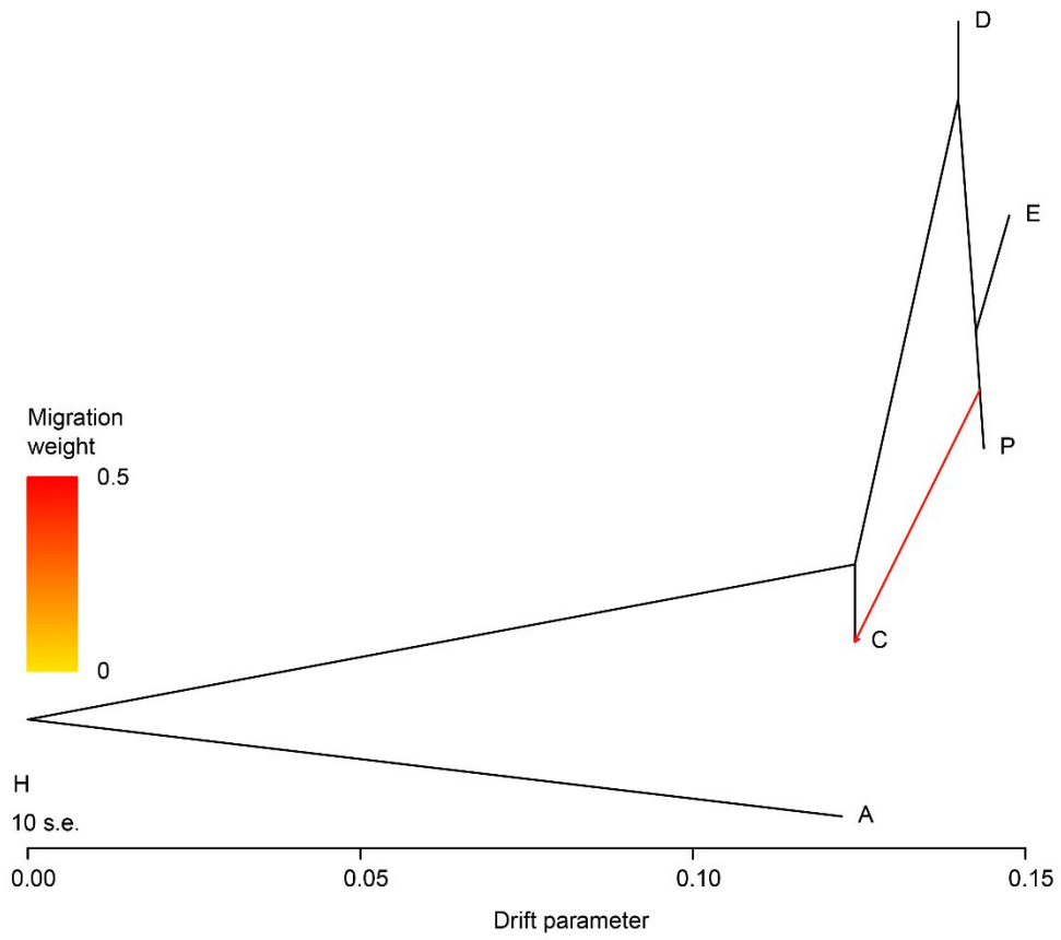
Supplemental Figure S5: Introgression among different populations of 1 Migration using TreeMix.
