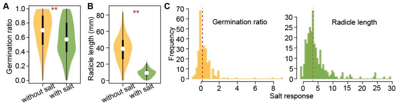
Figure S3. Germination ratio and radicle length under different salt conditions. (A-B) Distribution of germination ratio (A) and radicle length (B) under salinity (with salt) and the control group (without salt). Asterisks indicate significance levels based on paired Wilcoxon's test (**, P \leq 0.01 ). (C) The distributions of salt-responsive (SR) traits. The red dashed lines denote the median values.
