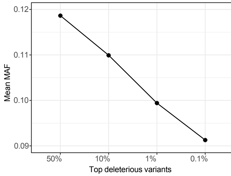
Figure S2. Mean minor allele frequency (MAF) of deleterious variants across different deleteriousness thresholds.
