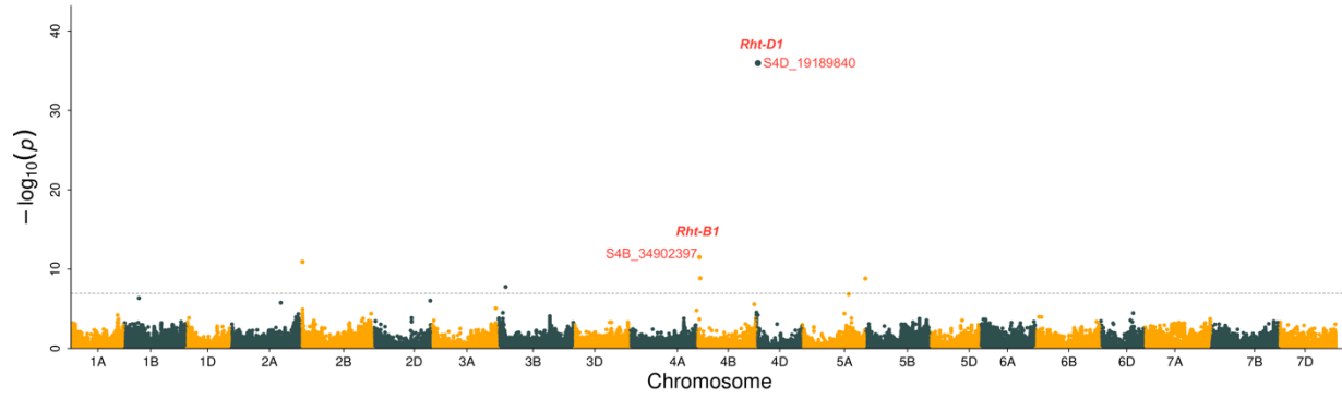
Fig. S4. Plant height GWAS using the FarmCPU model.
