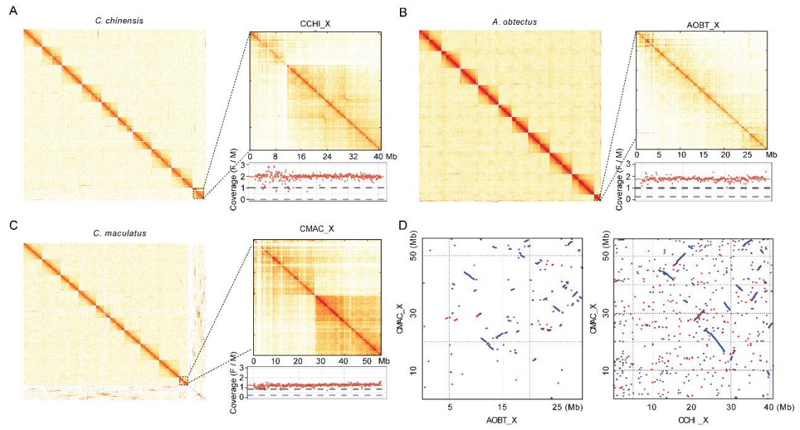
Figure S3. Independent Hi-C matrix and sequence alignment of X chromosomes. A-C, The X Hi-C matrix of C. chinensis (A), A. obtectus (B), and C. maculatus (C). D, Synteny dot plot of sequence alignment between seed beetles' X chromosomes. Forward orientation is visualized in red and reversed in blue.
