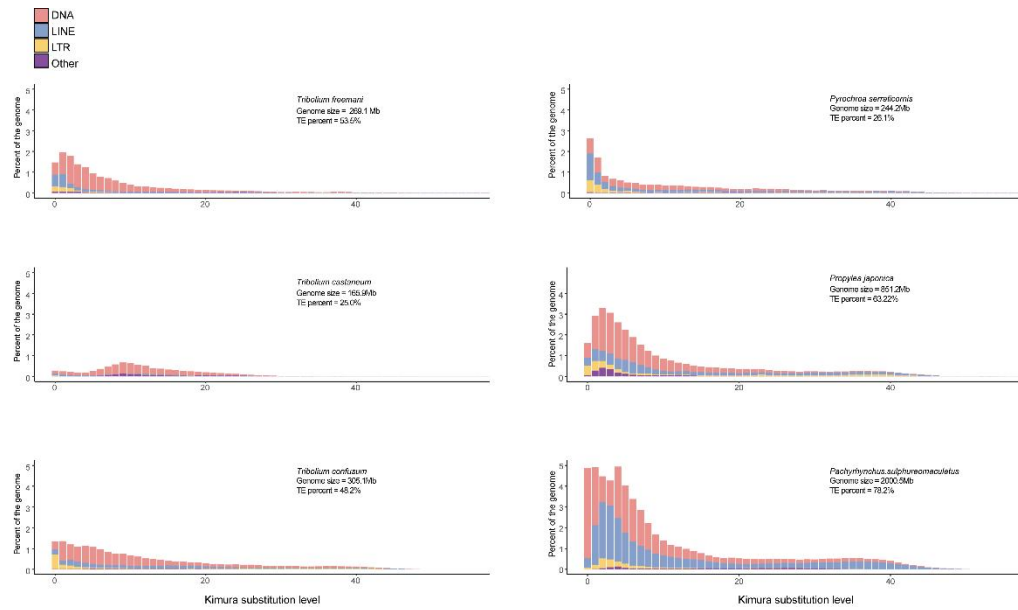
Figure S7. Insertion history of TEs among Coleoptera species. Vertical bars show the frequency of TE insertions during the evolution of species. The genome size and percentage of TEs in different species are marked in the graph.
