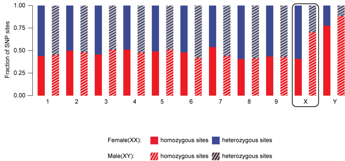
Figure S9. Allelic heterozygosity in C. chinensis . Female transcripts from X chromosome are overwhelmingly heterozygous, similar with autosomal transcripts, indicating that the X chromosome in females is biallelically expressed. Male transcripts from X chromosome are overwhelmingly homozygous, indicating that the X chromosome in males is monoallelically expressed.
