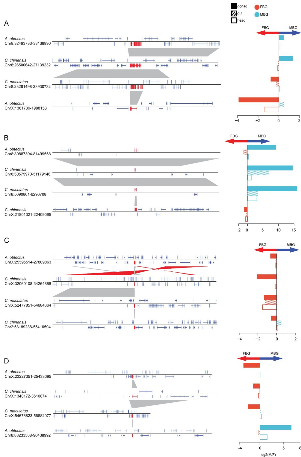
Figure S17. Examples of gene transfer resulting in genetic environmental changes and altered sex biased gene expression. A-B, Translocation of genes from autosomes to the X chromosome leads to biased expression toward females. C-D, Translocation of genes from the X chromosome to the autosome diminishes its initial female-biased expression pattern. The translocation genes are highlighted in red. The sex-biased expression pattern of these genes is assessed through their relative expression levels in different tissues and depicted using boxplots.
