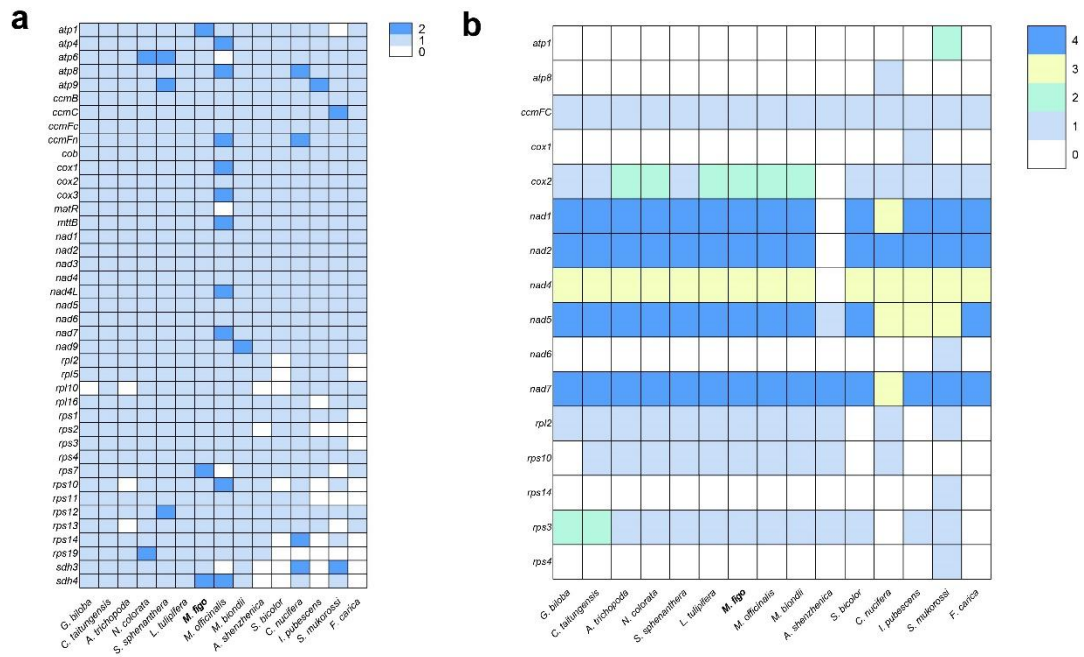
Figure S2 Heat maps of PCG and intron contents among 15 mitogenomes (a) Comparison of PCG contents among 15 mitogenomes. The gene numbers are shown on the top right. (b) Comparison of intron contents among 15 mitogenomes. The intron numbers are shown on the top right.
