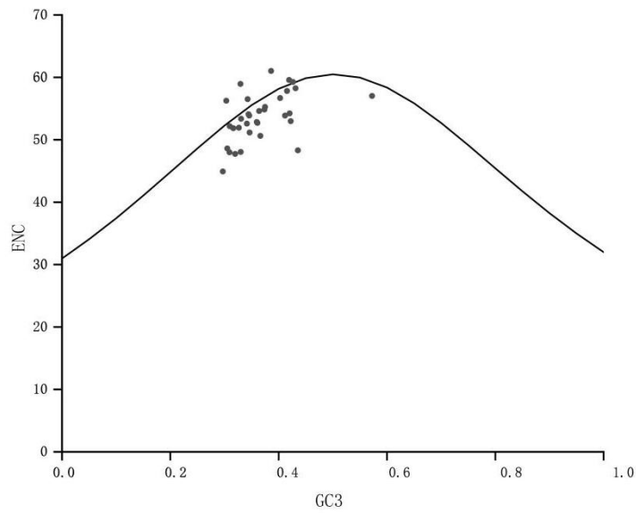
Fig. S1 ENC-plot against GC 3 of mitochondrial genome of S. alopecuroides . The solid lines represented the expected curve of positions of genes when the codon usage was only determined by the GC 3 composition.
