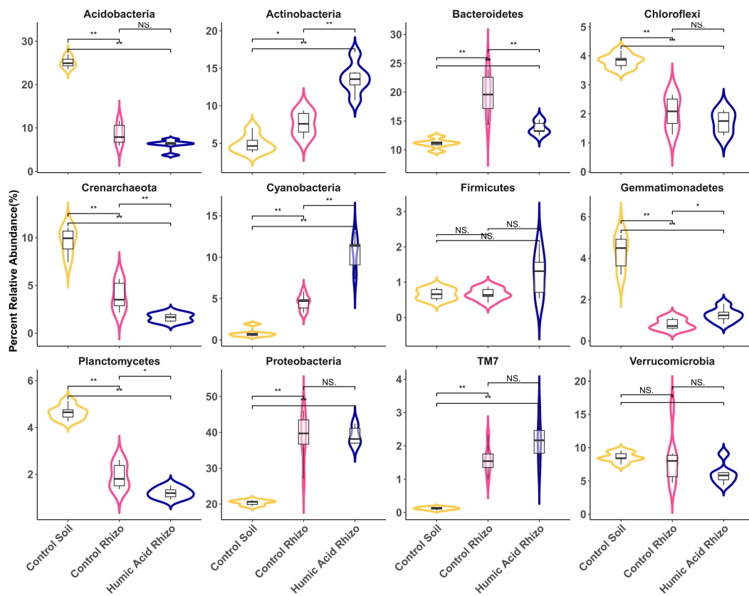
Figure S4. Wilcoxon Signed Rank Test for relative abundance of the abundant bacterial phyla in control soil, control rhizosphere and Humic Acid rhizosphere groups. * indicates P < 0.05 , ** indicates P < 0.01 , NS indicates not significant.
