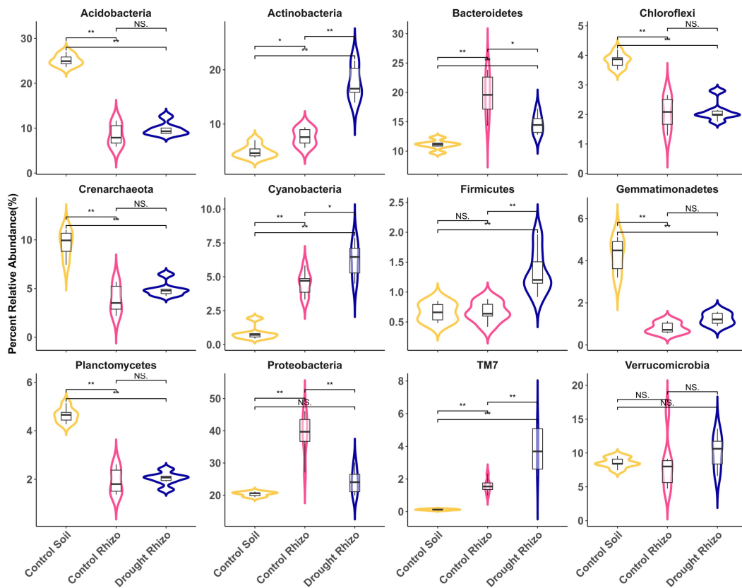
Figure S2. Wilcoxon Signed Rank Test for percent relative abundance of the abundant bacterial phylum in Control Soil, Control rhizosphere (Control Rhizo) and drought rhizosphere (Drought Rhizo) groups. * indicates P < 0.05 , ** indicates P < 0.01 , NS indicates not significant.
