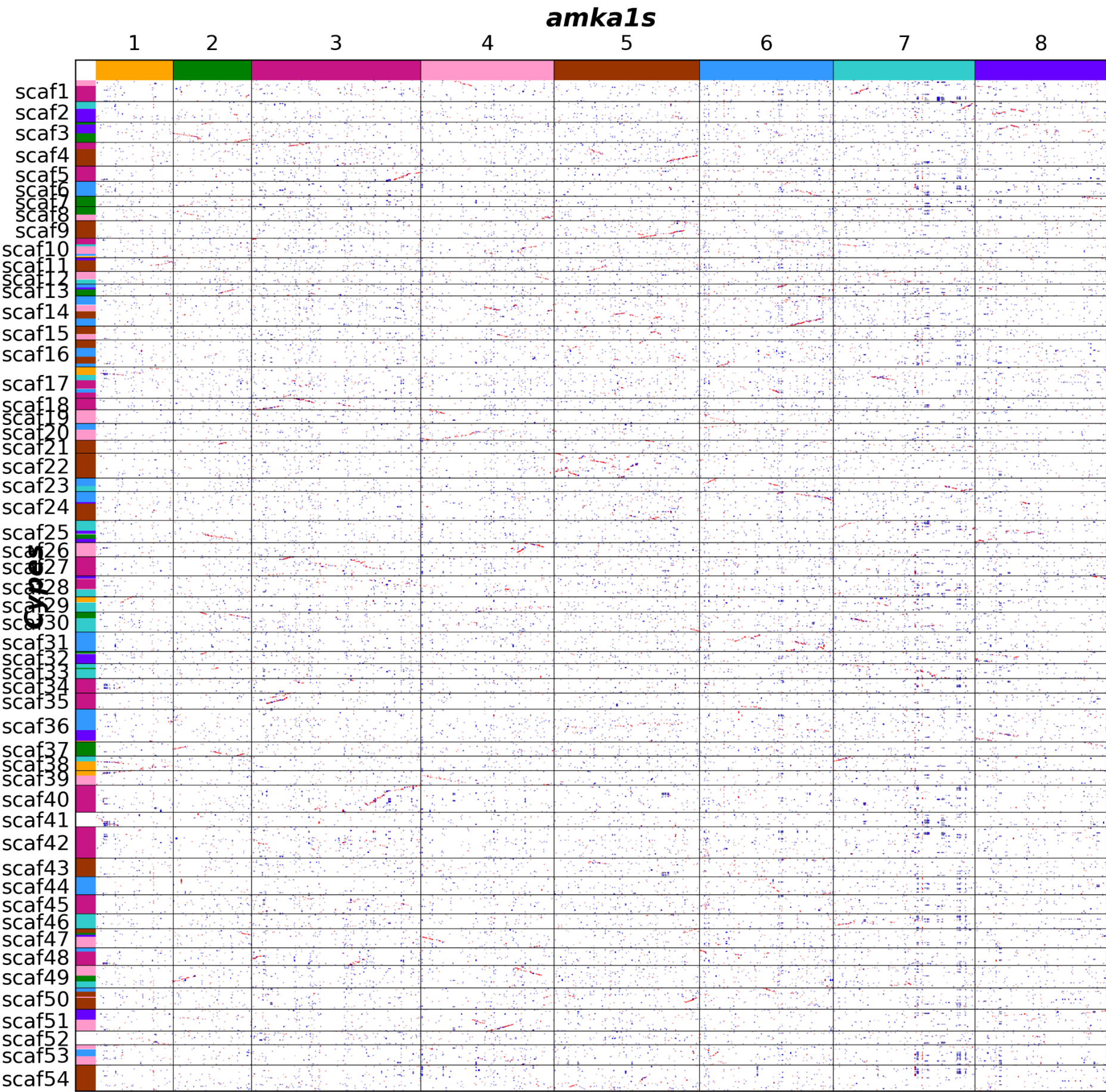
Supplementary Figure 6. Inferred karyotype evolution between AMAK and C. esculentus .
