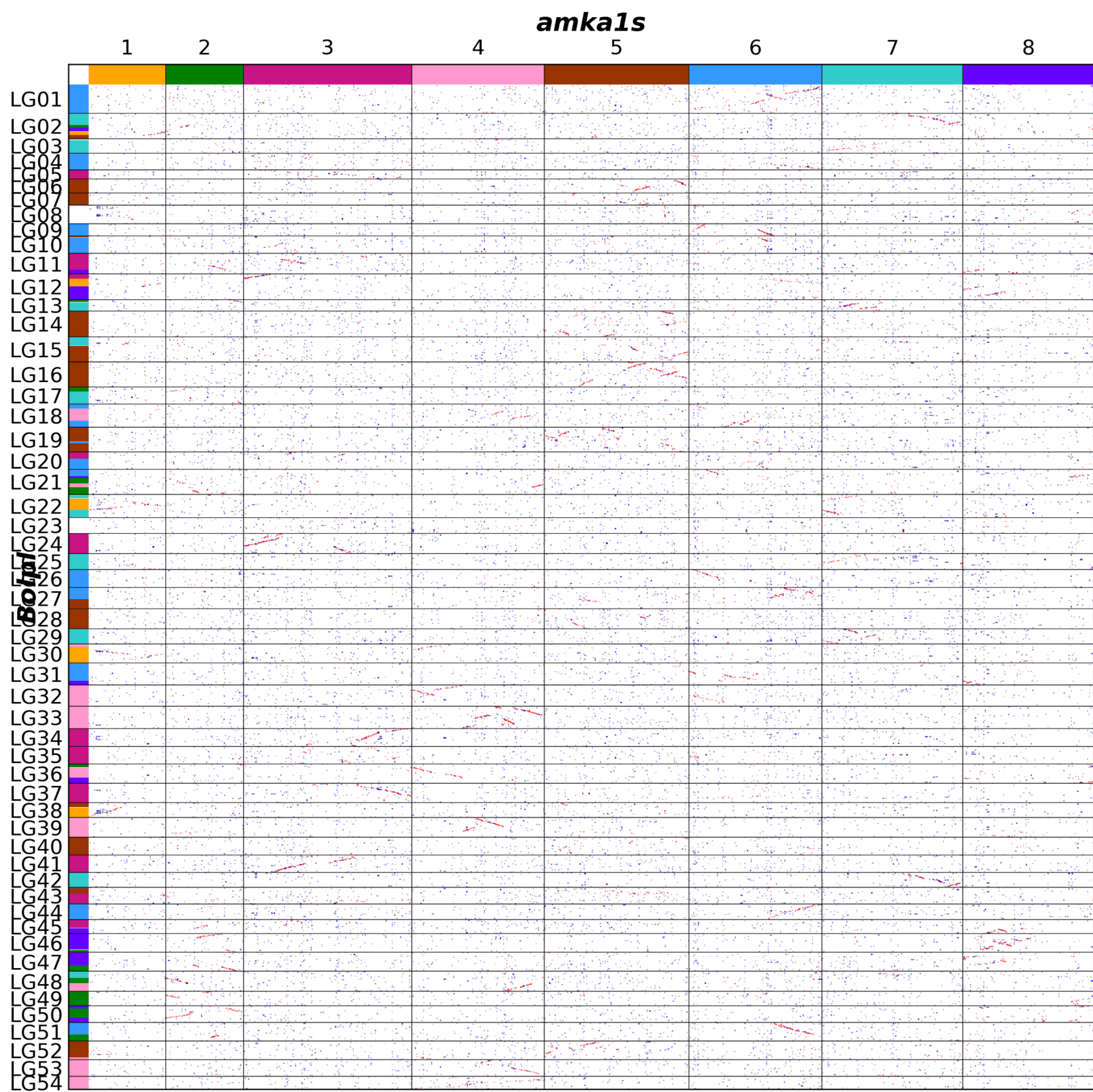
Supplementary Figure 5. Inferred karyotype evolution between AMAK and B. planiculmis .
