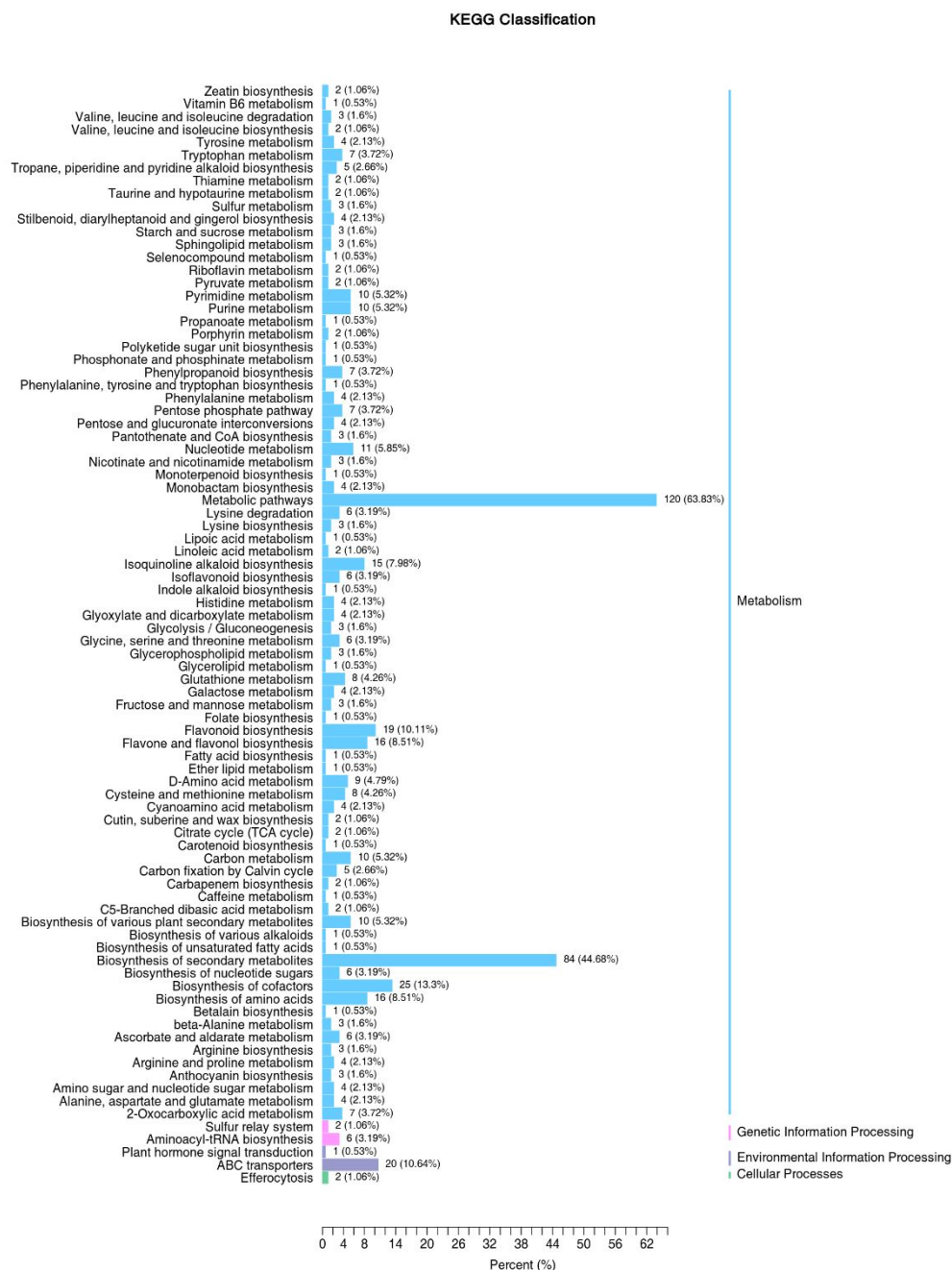
Fig. S5. KEGG classification of differential metabolites peel H2- flesh H2. The Y-axis shows the name of the KEGG pathway. The number of significant differential metabolites and the proportion of the total significant differential metabolites are shown next to the bar plot.
