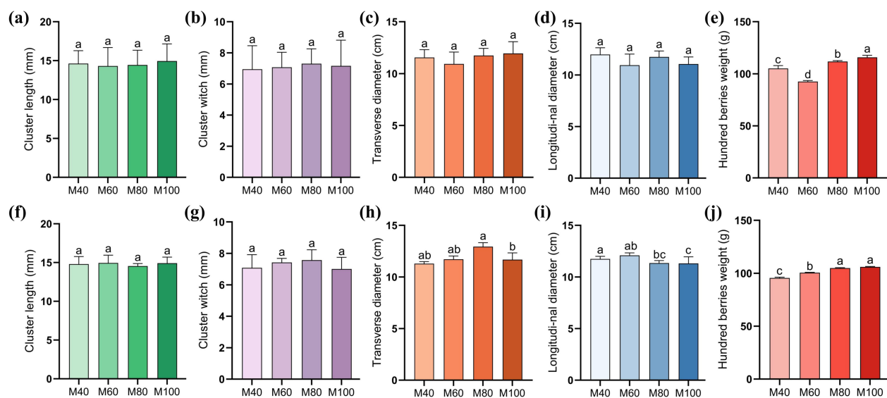
Fig. S2. Effect of different canopy thickness on basic physicochemical indexes of 'Merlot' grape.
